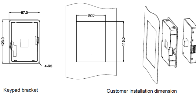
Keypad bracket
